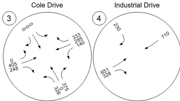
Figure 16 - Cole Drive Roundabout - Total AM Peak Hour Volumes
